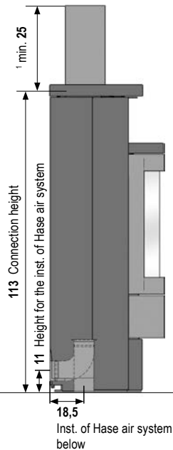
Side view Ceramic/Natural stone:
