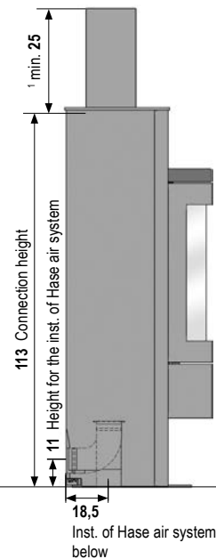
Side view Steel:
